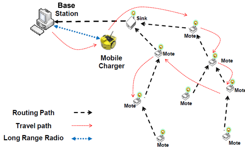
Figure 1.1 An example of joint routing and charging scheduling problem.
