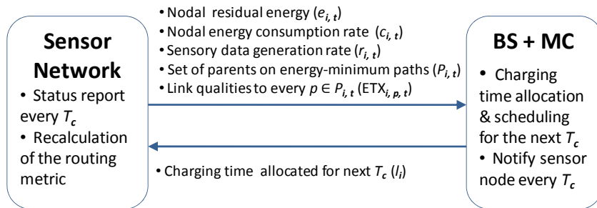
Figure 3.2 Overview of the proposed J-RoC scheme.
